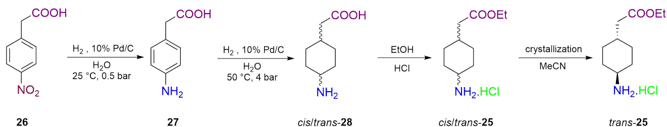
Scheme 15 Synthesis of trans -4-aminocyclohexylacetic acid ethyl ester.HCl ( trans -25)
