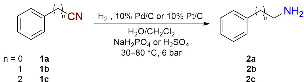
Scheme 2 Hydrogenation of benzonitrile and its homologues ( 1a–c ) to the corresponding primary amines ( 2a–c ) over Pd or Pt catalyst
