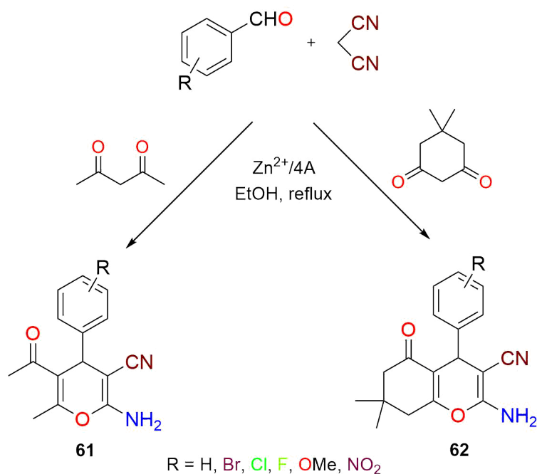
Scheme 31 Multicomponent reaction with acetylacetone or dimedone using a Zn 2+ /4A catalyst
