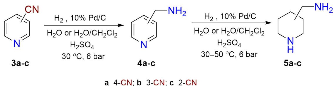
Scheme 3 Selective, Pd-catalyzed hydrogenation of 4-, 3- and 2-pyridinecarbonitriles ( 3a-c ) to 4-, 3- and 2-(aminomethyl)pyridines ( 4a-c ) or 4-, 3- and 2-(aminomethyl)piperidines ( 5a-c )
