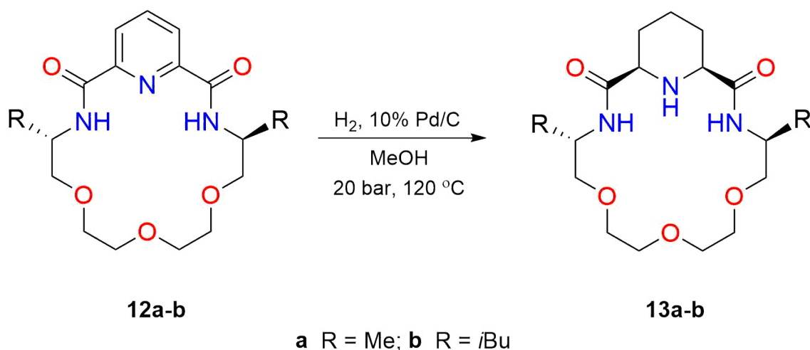
Scheme 8 Synthesis of enantiopure cis -piperidino-18-crown-6-ethers ( 13a-b ) by Pd-catalyzed hydrogenation of pyridino-18-crown-6-ethers ( 12a-b )
