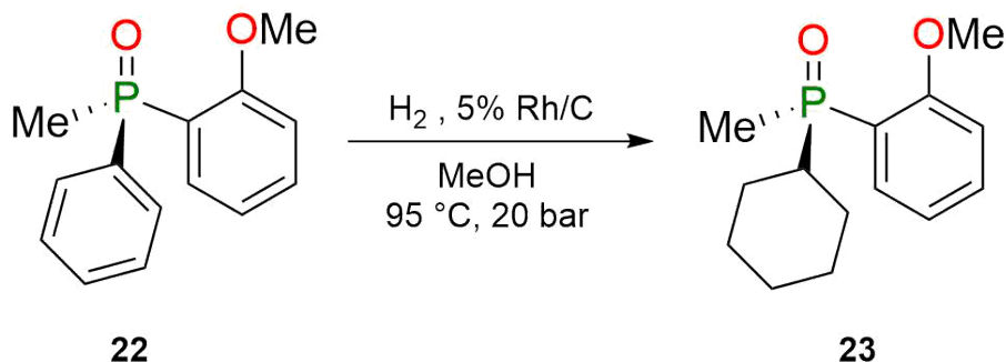
Scheme 13 Selective, Rh-catalyzed hydrogenation of a phenylphosphine oxide derivative ( 22 ) to the corresponding cyclohexyl one ( 23 )
