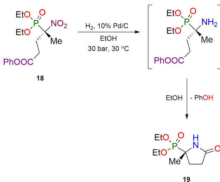
Scheme 11 Pd-catalyzed hydrogenation of an \alpha -nitrophosphonate Michael adduct ( 18 ) to a cyclic \alpha -aminophosphonate derivative ( 19 )
