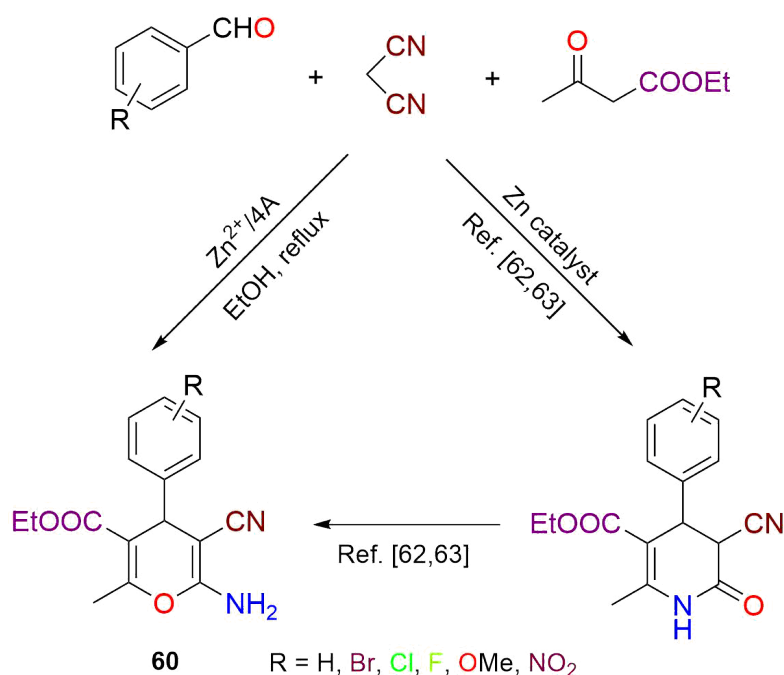
Scheme 30 Zn-catalyzed synthesis of 4 H -pyran derivatives ( 60 )
