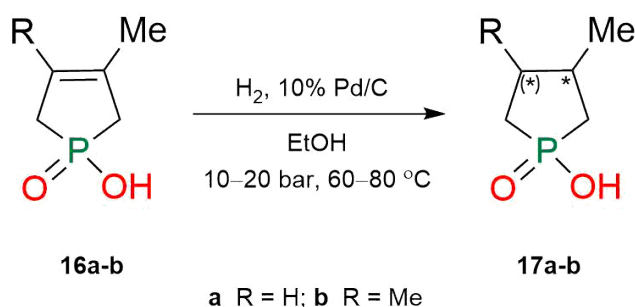
Scheme 10 Hydrogenation of 1-hydroxy-3-phospholene 1-oxides ( 16a-b ) to the corresponding 1-hydroxy-3-phospholane 1-oxides ( 17a-b ) with Pd/C
