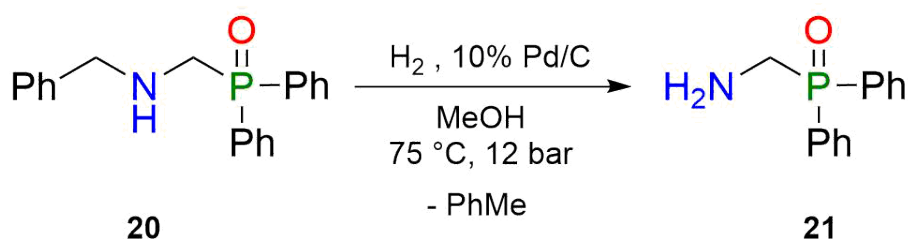
Scheme 12 Hydrogenolysis of ( N -benzylaminomethyl)diphenylphosphine oxide ( 20 ) to (aminomethyl)diphenylphosphine oxide ( 21 ) over Pd/C
