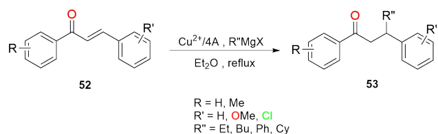
Scheme 24 Cu-catalyzed 1,4-addition of Grignard compounds to chalcones ( 52 )
