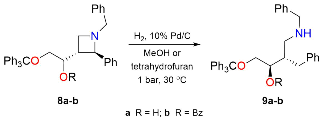
Scheme 6 Selective ring opening of trans - N -benzylazetidines ( 8a-b ) to anti - N -benzylamino derivatives ( 9a-b ) over Pd/C
