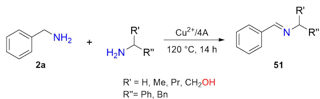
Scheme 23 Transformation of benzylamine ( 2a ) into imines ( 51 ) with a \text{Cu}^{2+}/4\text{A} catalyst
