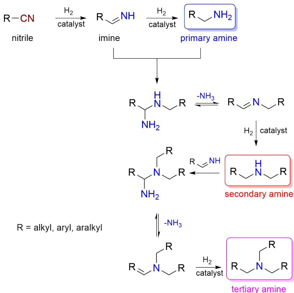
Scheme 1 General scheme for the catalytic hydrogenation of nitriles
