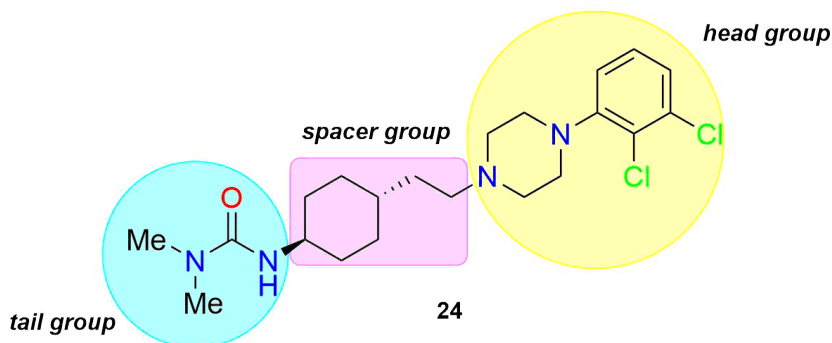
Scheme 14 Structure of cariprazine ( 24 )
