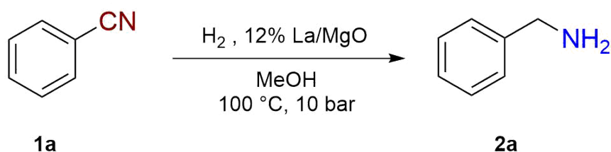
Scheme 4 Hydrogenation of benzonitrile ( 1a ) to benzylamine ( 2a ) over a 12% La/MgO catalyst
