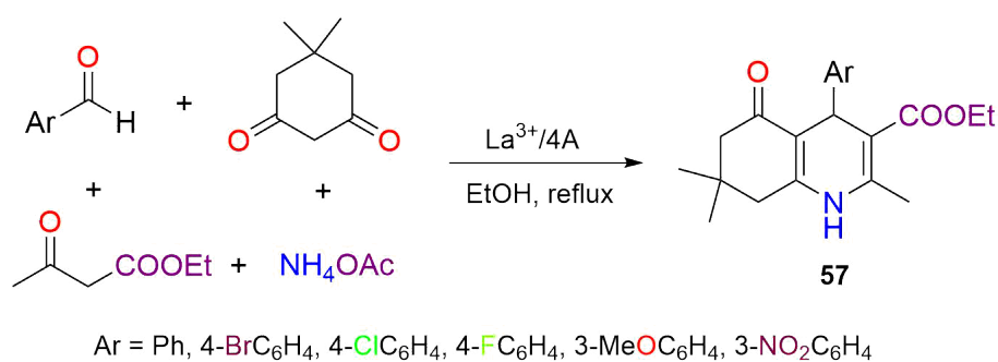
Scheme 27 Synthesis of polyhydroquinoline derivatives ( 57 ) over a \text{La}^{3+}/4\text{A} catalyst
