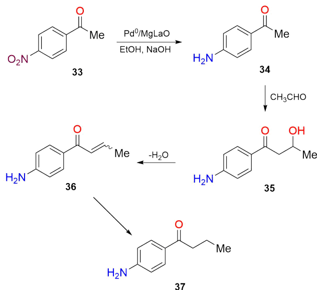
Scheme 17 Mechanism of the chain elongation reaction of 4-nitroacetophenone ( 33 )
