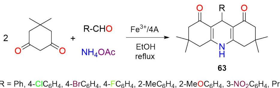
Scheme 32 Fe-catalyzed synthesis of acridindione derivatives ( 63 )
