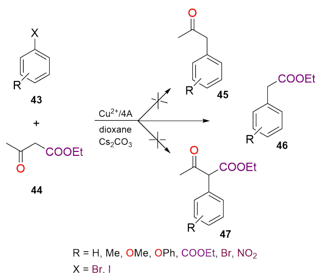
Scheme 21 Selective synthesis of arylacetic acid ethyl esters ( 46 ) in the presence of a \text{Cu}^{2+}/4\text{A} catalyst
