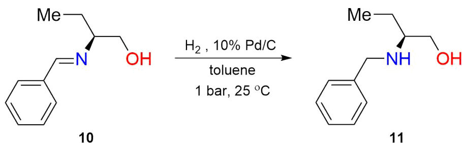
Scheme 7 Hydrogenation of a Schiff base, ( S )-(+)-2-( N -benzylideneamino)butan-1-ol ( 10 ), to ( S )-(+)-2-( N -benzylamino)butan-1-ol ( 11 ) over Pd/C
