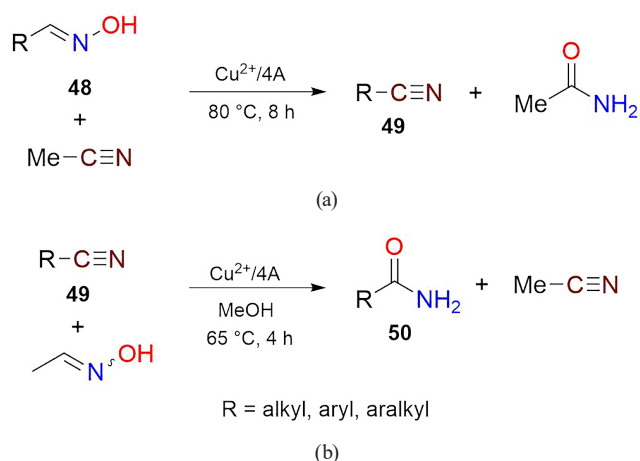
Scheme 22 Cu-catalyzed oxime–nitrile (a) and nitrile–amide (b) transformation
