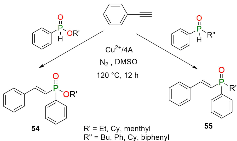
Scheme 25 Conversion of H -phosphinates and phosphine oxides to ( E )-alkenylphosphinates ( 54 ) and ( E )-alkenylphosphine oxides ( 55 )
