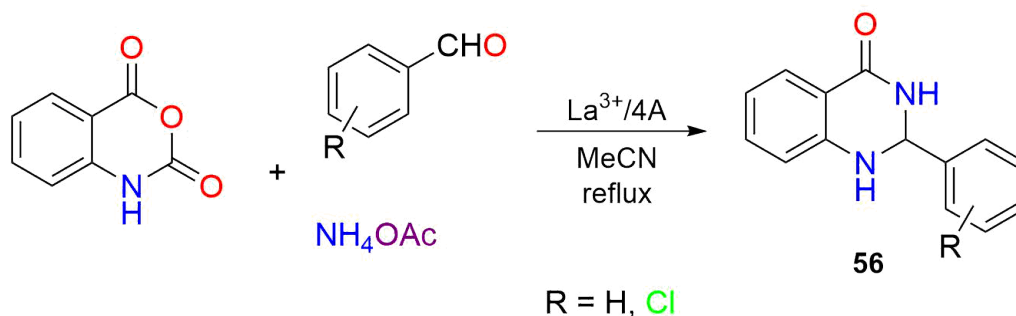
Scheme 26 Synthesis of 2,3-dihydroquinazolin-4(1 H )-ones ( 56 ) using a \text{La}^{3+}/4\text{A} catalyst
