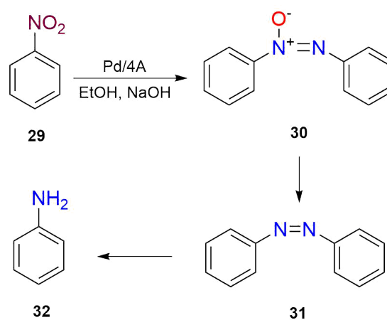
Scheme 16 Selective transfer hydrogenation of nitrobenzene (29)
