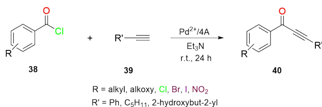
Scheme 18 Acyl Sonogashira reaction of benzoyl chloride derivatives ( 38 ) and alkynes
