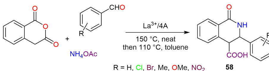
Scheme 28 La-catalyzed multicomponent reaction yielding tetrahydro-isoquinolonic acid derivatives ( 58 )
