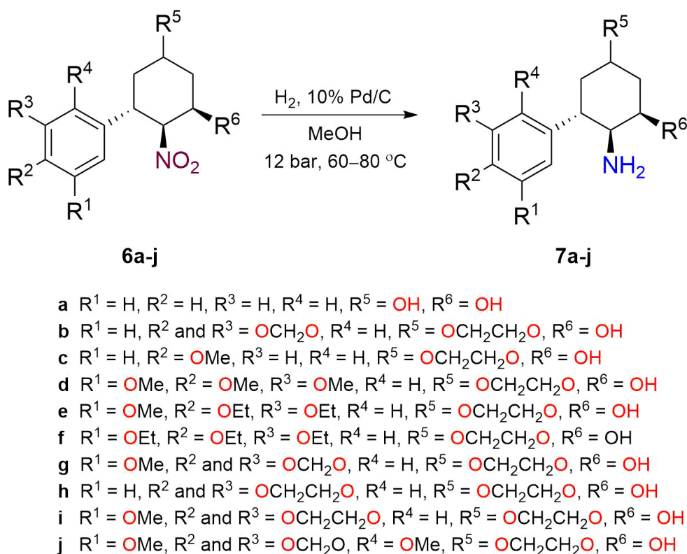
Scheme 5 Hydrogenation of ( \pm )- trans -4-nitro-5-phenylcyclohexane-1,3-diol and its derivatives ( 6a-j ) to the corresponding cyclohexylamines ( 7a-j ) over palladium
