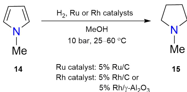
Scheme 9 Saturation of 1-methylpyrrole ( 14 ) to 1-methylpyrrolidine ( 15 ) over supported Ru or Rh catalyst
