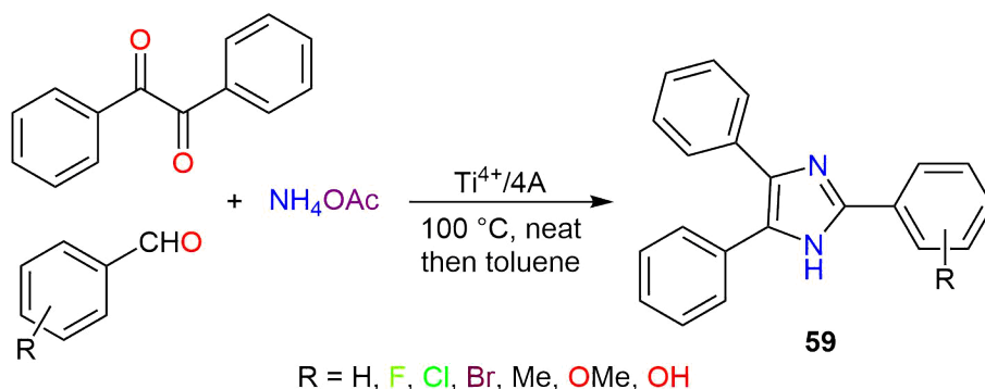
Scheme 29 Ti-catalyzed multicomponent synthesis of 2,4,5-triarylimidazole derivatives ( 59 )
