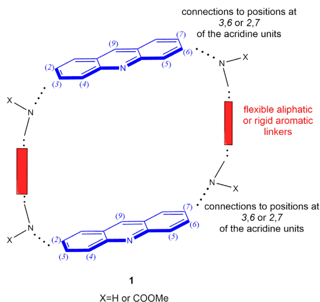
Fig. 1 Cyclo-bis-intercorporations containing acridine subunits linked by different spacers as most commonly used bisacridino-macrocycles with a nucleic acid-specific applicability
