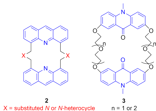
Fig. 2 Macrocyclic analogues containing two acridine or two acridone units (made by Panna Vezse based on the synthesis in [14–16])
