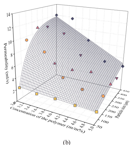
Fig. 4 Permeability of the scaffolds plotted against the concentration of the solution of the polymer (a) and against the concentration and the average size of particles (b)
