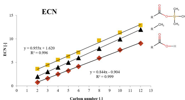
Fig. 3 Relationship of ECN and actual carbon number, red: straight chain fatty acids ( \text{C}_2-\text{C}_{12} ), yellow: trimethylsilyl derivatives of straight chain fatty acids ( \text{C}_2-\text{C}_{12} ), black: alkanes (theoretical values)
