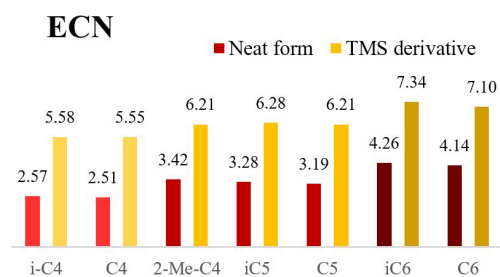
Fig. 4 ECN of carboxylic acid isomers ( \text{C}_4-\text{C}_6 ), neat and TMS derivatized form
