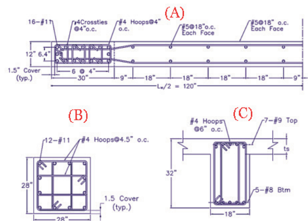
Fig. 5 The specifications of the member cross sections: (A) wall, (B) column, and (C) beam [30]
