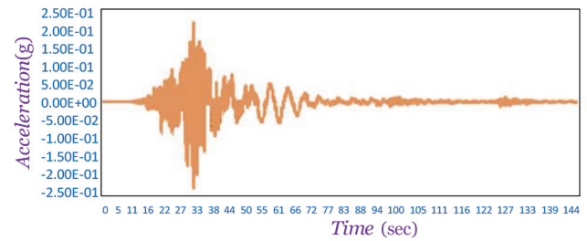
Fig. 17 Horizontal component of the main earthquake of CACS station in N50W direction
