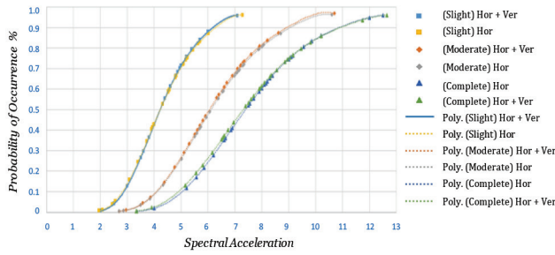
Fig. 30 Fragility curve of the IR_3S_LO structure by applying horizontal components and by applying horizontal + vertical components of main earthquakes
