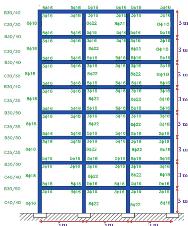
Fig. 3 Regular 8-story frame and its specifications [4]
