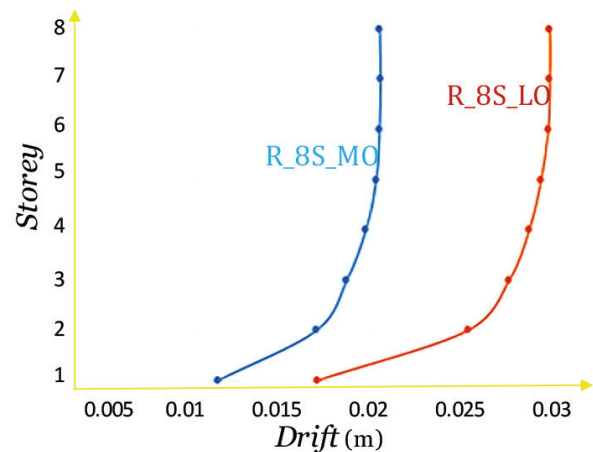
Fig. 29 Drift of the floors of the R_8S_LO structure under spectral acceleration of 4.5
