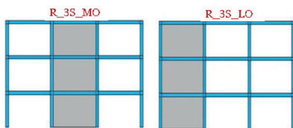
Fig. 10 The regular 3-story reinforced concrete structure with a shear wall in the middle and left openings
