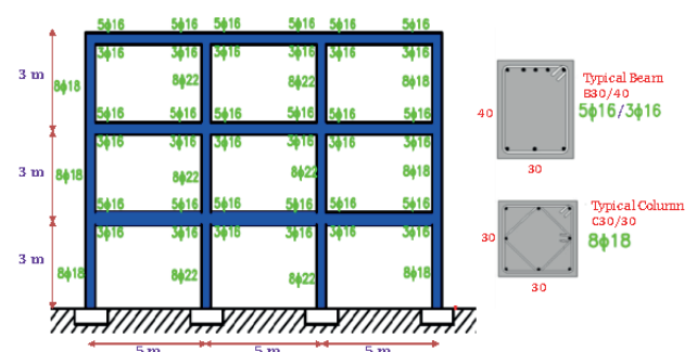
Fig. 1 Regular 3-story frame and its specifications
