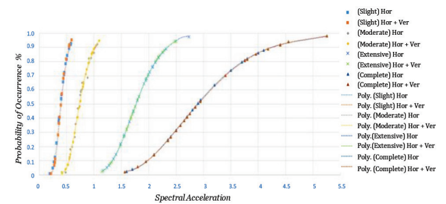
Fig. 35 Fragility curve of the IR_3S_RO structure by applying horizontal components and by applying horizontal + vertical components of seismic sequences
