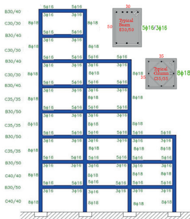
Fig. 4 Irregular 8-story frame and its specifications [4]
