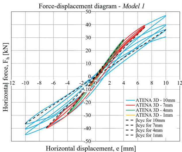
Fig. 24 Force-displacement diagram – reduction factors
