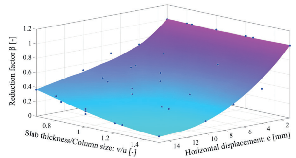
Fig. 18 Graph of the reduction factor ( \beta ) – grid ratio: 0.50
