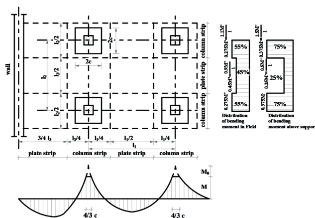
Fig. 2 Definition of the column and plate strip [7]
