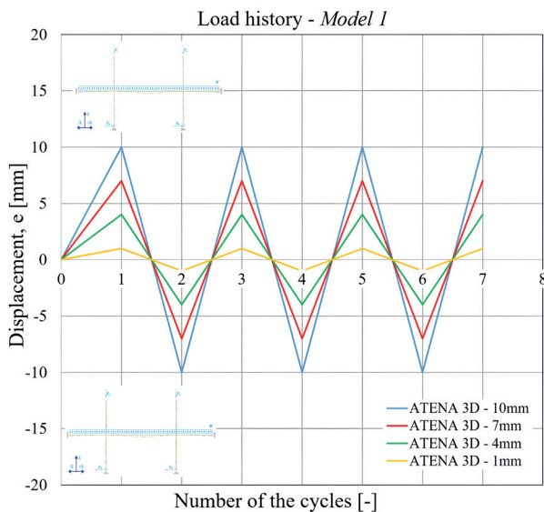
Fig. 22 Load history for cyclic analyses
