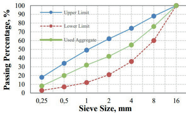
Fig. 1 The sieve analysis of aggregates [23]
