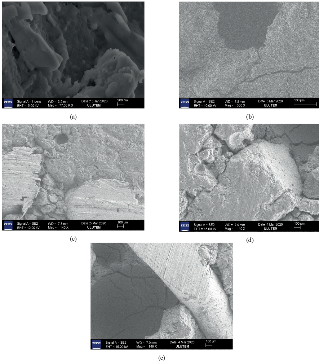
Fig. 5 SEM images of rubberized GC slabs with/out SF; (a) GS, (b) GS-7.5FCR-7.5CCR, (c) GS-1.0SF-7.5FCR-7.5CCR, (d) GS-15TCR, (e) GS-1.0SF-10TCR
