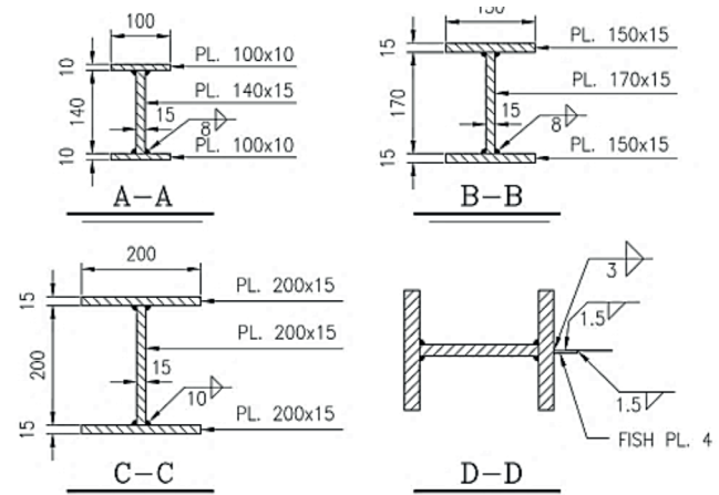
Fig. 2 HBE and VBE sections (mm): (a) Section top HBEs, (b) Section VBEs, (c) Bottom HBE, and (d) Details of fish plate connection to the boundary elements. (Note: HBE: Horizontal boundary element; VBE: Vertical boundary element)
