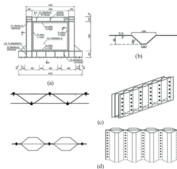
Fig. 1 Specification of specimens: Specification of the (a) frames (horizontal boundary elements (HBEs) and vertical boundary elements (VBEs) specimens and web-plate of the SPSW specimen (mm), (b) web-plate of the CSPSW specimen (mm), (c) web-plate of the SCSSPW specimen, and (d) web-plate of the CSCSPW specimen
