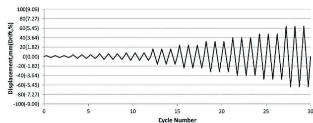
Fig. 5 Loading pattern
