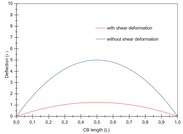
Fig. 8 Deflection v(x)/[M_0 - L^2/E \cdot b^4] vs. the length of the composite beam with/without the shear deformation
