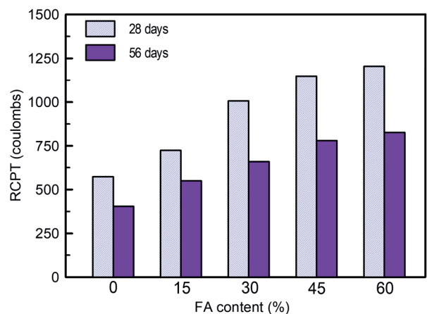
Fig. 16 Effect of FA content on RCPT
