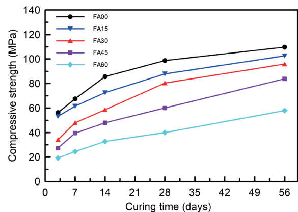
Fig. 7 Effect of FA content on compressive strength
