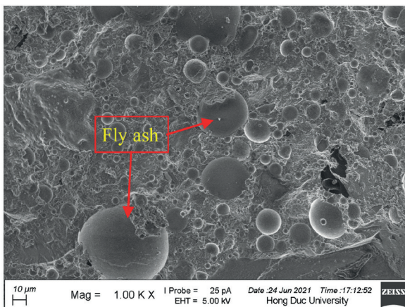
Fig. 11 SEM micrograph of FA60
