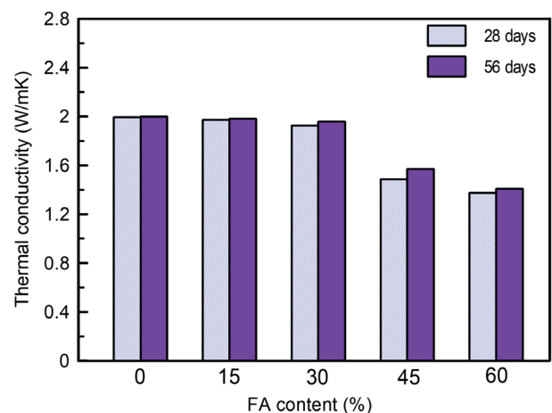
Fig. 18 Effect of FA content on thermal conductivity
