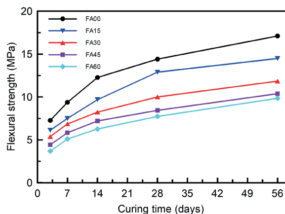
Fig. 8 Effect of FA content on flexural strength
