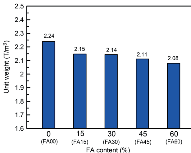
Fig. 6 Effect of FA content on unit weight
