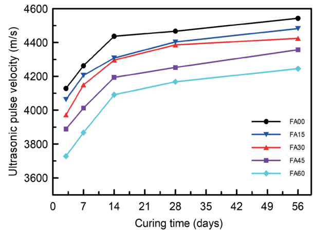
Fig. 12 Effect of FA content on UPV
