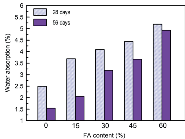
Fig. 15 Effect of FA content on water absorption
