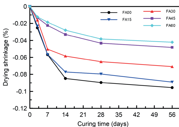
Fig. 17 Effect of FA content on drying shrinkage
