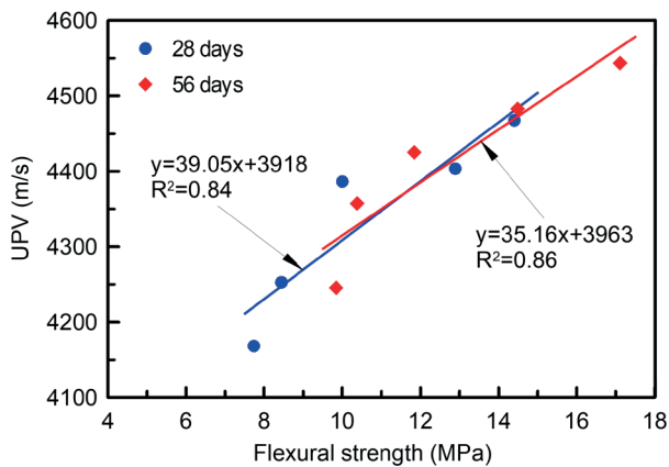
Fig. 14 Correlation between UPV and flexural strength
