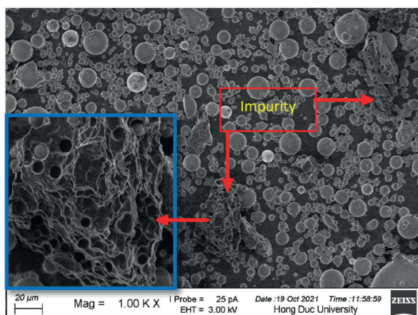
Fig. 5 SEM observation of fly ash
