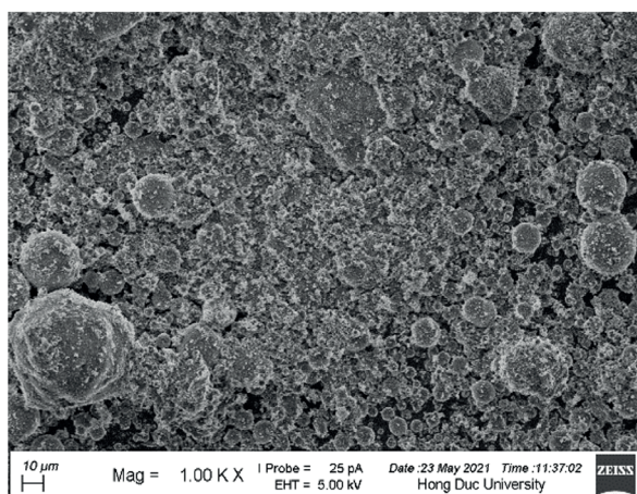
Fig. 4 SEM observation of silica fume
