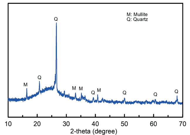
Fig. 2 XRD pattern of FA
