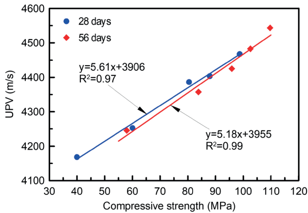
Fig. 13 Correlation between UPV and compressive strength
