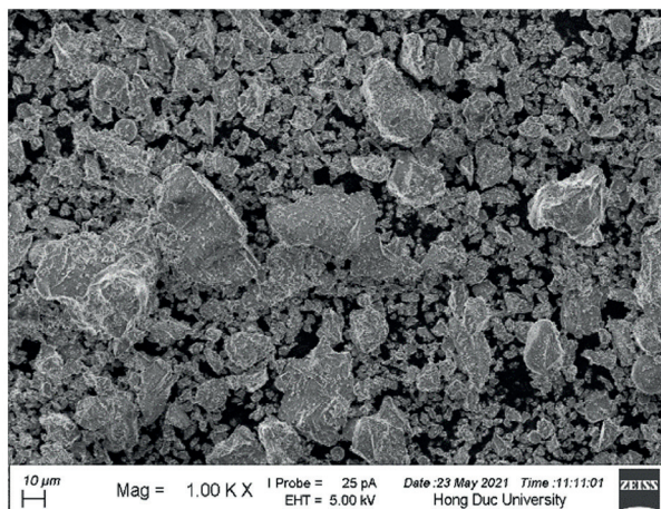
Fig. 3 SEM observation of cement
