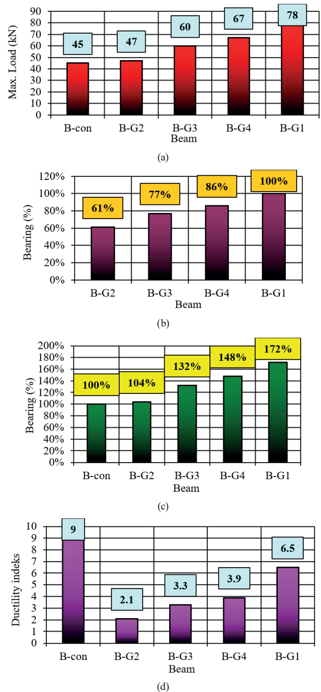
Fig. 5 Strength and ductility of the tested specimens: (a) max. strength, (b) strength related to the B-G1 (%), (c) strength related to the B-con (%), (d) ductility index
