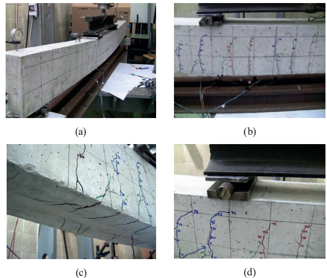
Fig. 8 (a) B-G1, beam deflection ( \Delta_{\max} = 78 mm), (b) B-G1, max. crack width ( \delta_{\max} = 3.2 mm), (c) B-G1, beam failure caused by the loss of concrete-epoxy connection, (d) B-G1, beam concrete crushing in the area of force application at the beam failure
