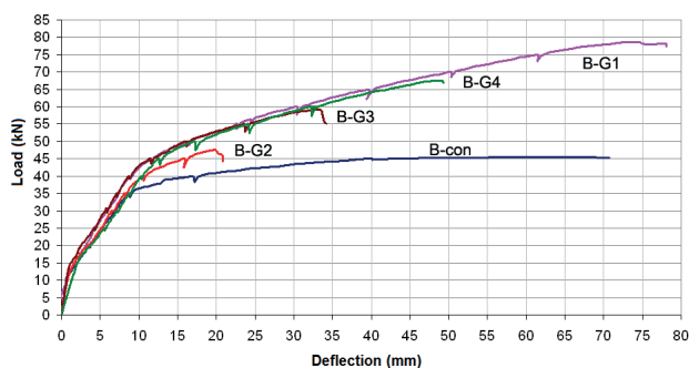
Fig. 4 Load-deflection diagrams for different variants of splicing of GFRP reinforcement
