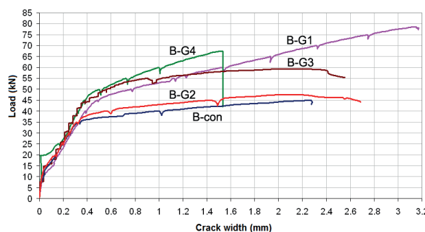
Fig. 12 Crack width diagrams for all tested beam specimens
