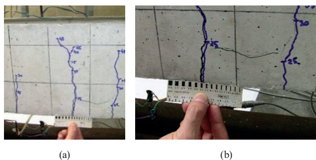
Fig. 9 Crack pattern at the beam B-G2 (cut off, without bypassing), dominant crack at the cut off: (a) general view, (b) detail view
