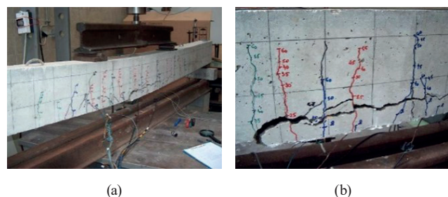
Fig. 11 Crack distribution at beam B-G4 (bypassing 40Ø): (a) general view, (b) detail view
