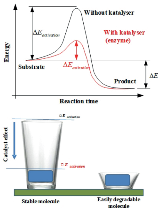
Fig. 2 Representations of the enzyme catalysis process
