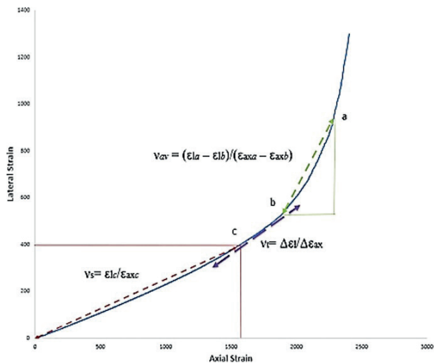
Fig. 1 Schematic calculation of (a) secant Poisson's ratio ( v_s ), (b) tangent Poisson's ratio ( v_t ) and (c) average Poisson's ratio ( v_{av} ) of intact rock [5]
