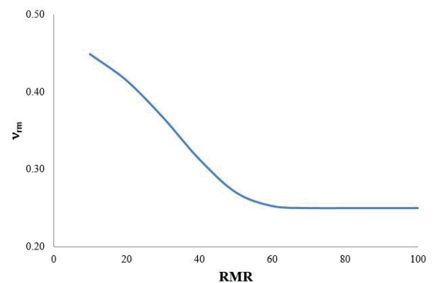
Fig. 11 Poisson's ratio of rock mass ( v_{rm} ) as a function of the RMR , independent of the strength of intact rock (Eq. (9))
