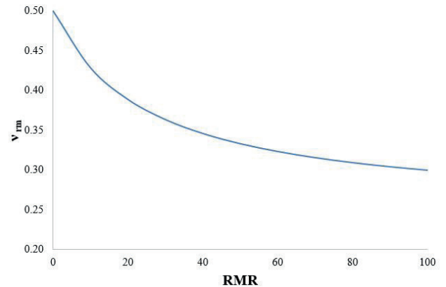
Fig. 17 Poisson's ratio of the rock mass ( v_{rm} ) in the function of Rock Mass Rate ( RMR ) (Eq. (19))
