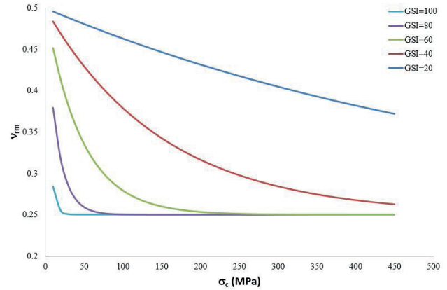
Fig. 13 Poisson's ratio of the rock mass ( \nu_{rm} ) as a function of uniaxial compressive strength ( \sigma_c ) for different values of GSI (Eq. (15))
