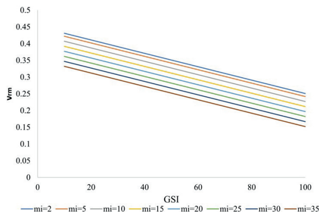
Fig. 22 Poisson's ratio ( \nu_m ) in function of GSI in case of different Hoek-Brown constants (Eq. (22))
