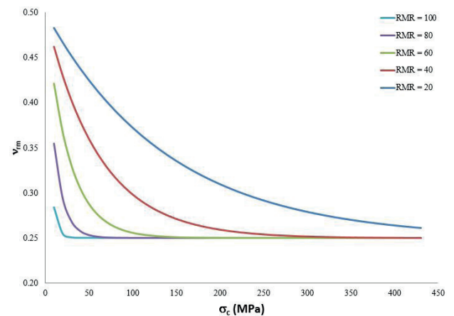
Fig. 10 Poisson's ratio of rock mass ( v_{rm} ) as a function of uniaxial compressive strength for different values of RMR (Eq. (6))
