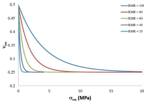
Fig. 9 Poisson's ratio of rock mass ( v_{rm} ) as a function of the rock mass strength for different values of RMR (Eq. (6))
