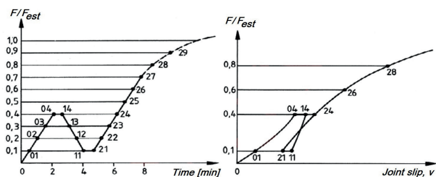
Fig. 3 Loading procedure for push-out test [32]
