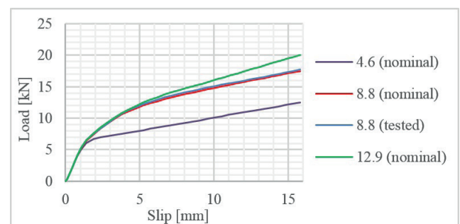
Fig. 18 Load-slip curves for different grades of bolt material
