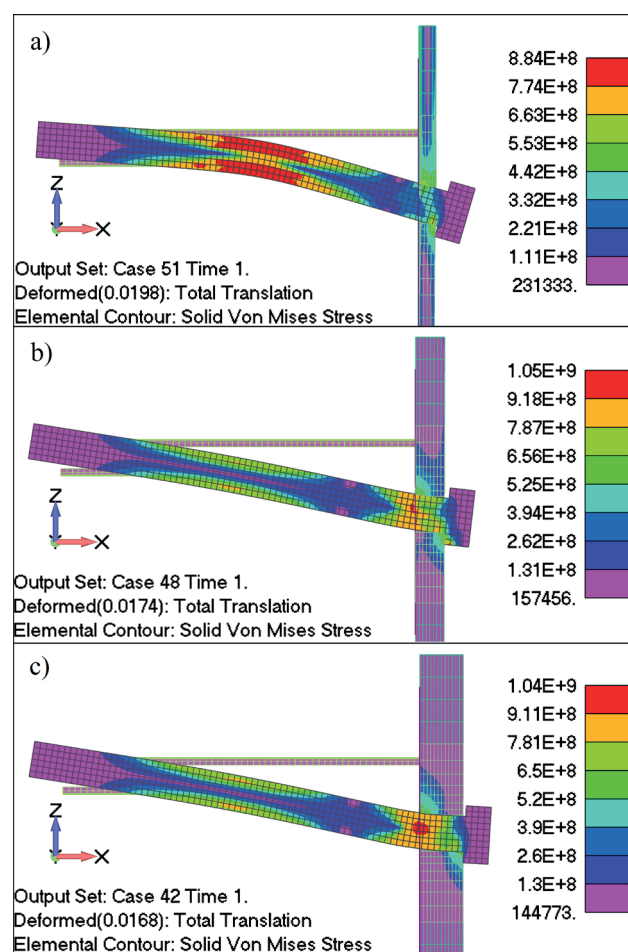
Fig. 26 Failure modes without rope effect: (a) t = 4 mm, (b) t = 8 mm, (c) t = 12 mm
