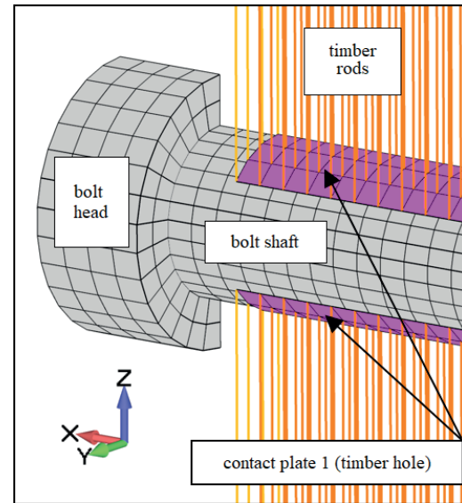
Fig. 10 Bolt and bolt hole – modelling detail
