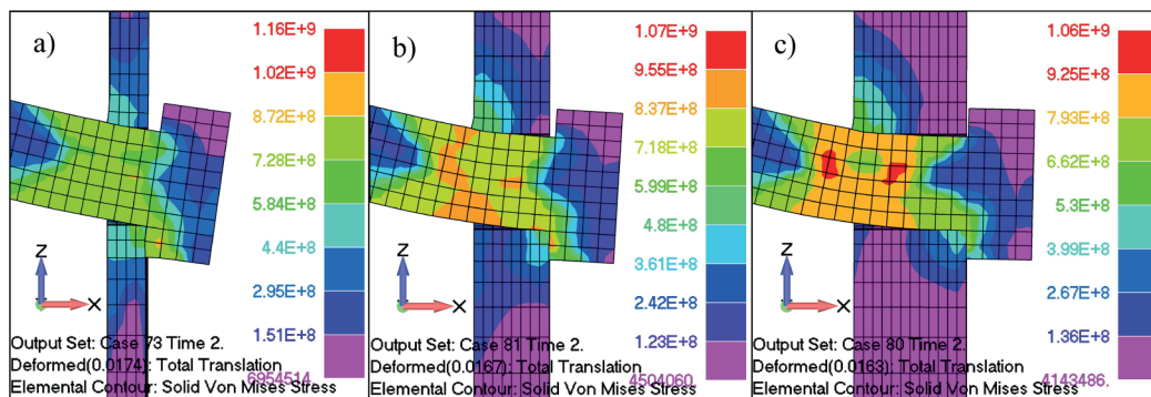
Fig. 24 Rotation of the bolt head for different steel web thicknesses; (a) t = 4 mm, (b) t = 8 mm, (c) t = 12 mm
