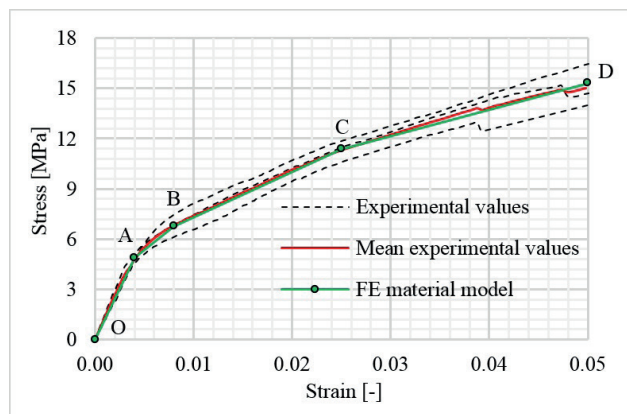
Fig. 11 Stress-strain curves for "timber under nut" element
