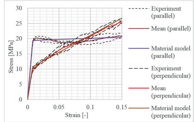
Fig. 9 Diagrams of the embedment pressure: experimental data and bilinear material law
