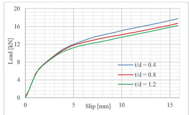
Fig. 22 Behavior of the connection as a function of the steel profile web thickness: load-slip curves
