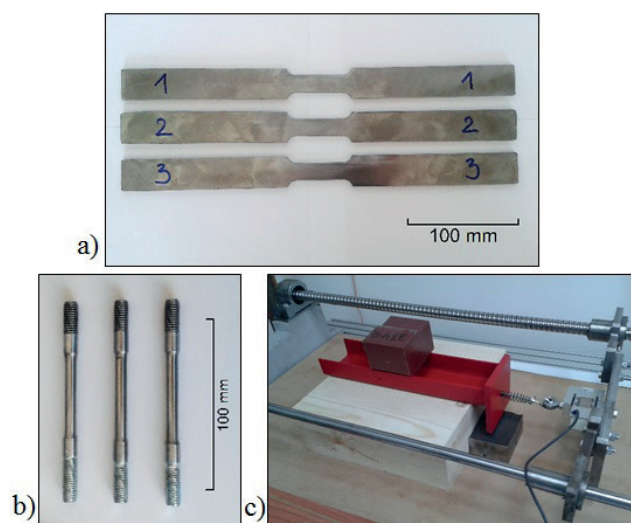
Fig. 6 Specimens: (a) steel S275 for tensile test, (b) steel 8.8 for tensile test, (c) steel profile-CLT panel for friction test
