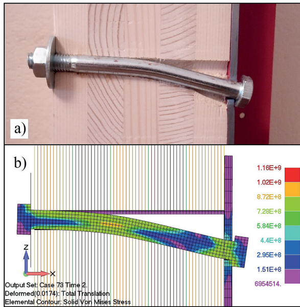
Fig. 16 Model validation – failure mode; (a) experiment; (b) numerical analysis (bolt von Mises stresses and deformation)
