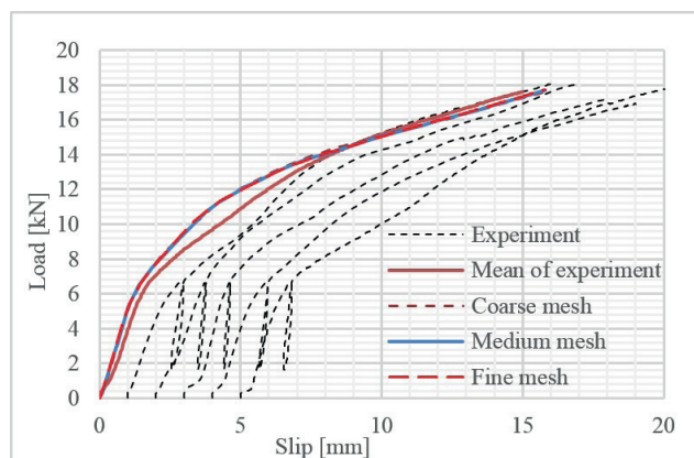
Fig. 15 Results of the numerical analysis for different FE mesh densities and results of the experimental analysis
