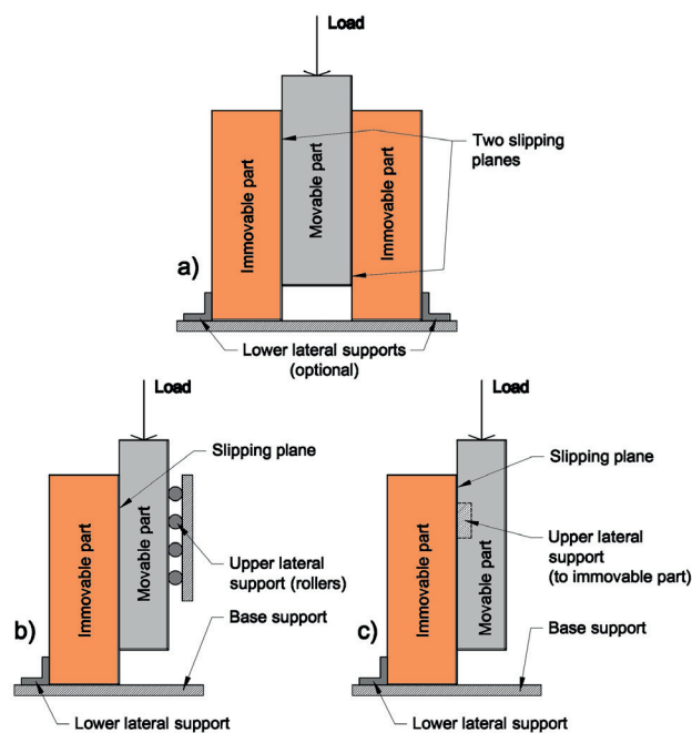
Fig. 1 Types of push-out test: (a) symmetrical, (b) asymmetrical with lateral support of the movable part, (c) asymmetrical with lateral support of the immovable part
