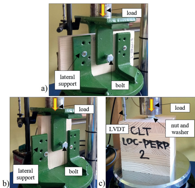
Fig. 5 (a), (b) Examination of timber under embedment pressure; (c) examination of the timber resistance at washer imprinting
