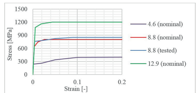
Fig. 17 Stress-strain curves for different grades of bolt material
