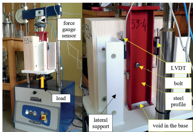
Fig. 4 Push-out specimen with measuring instrumentation
