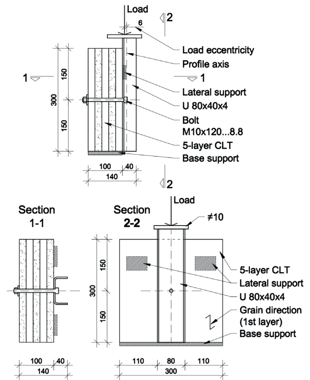
Fig. 2 Details of the push-out test specimen with supports (measures in mm)
