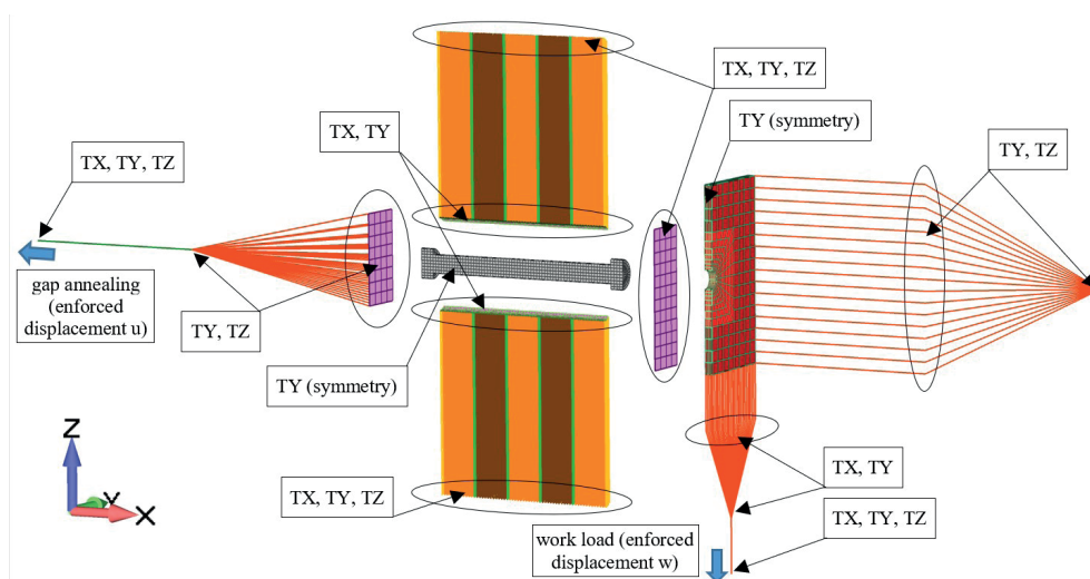
Fig. 12 Loading and boundary conditions (TX, TY, TZ – restrained displacements)
