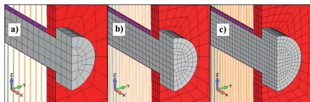
Fig. 14 Mesh density; (a) coarse, (b) medium, (c) fine
