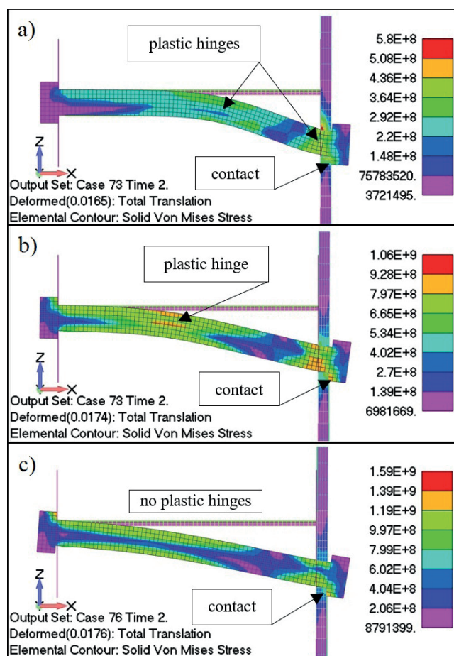
Fig. 19 Failure modes for different bolt grades; deformation and von Mises stress contours: a) 4.6, b) 8.8, c) 12.9
