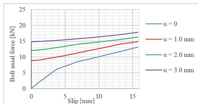
Fig. 21 Bolt axial force-slip diagram depending on the bolt-pretension
