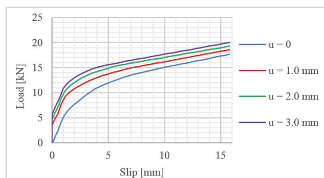
Fig. 20 Load-slip diagram of the connection depending on the bolt-pretension
