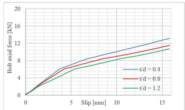
Fig. 23 Behavior of the connection as a function of the steel profile web thickness: bolt axial force-slip diagram
