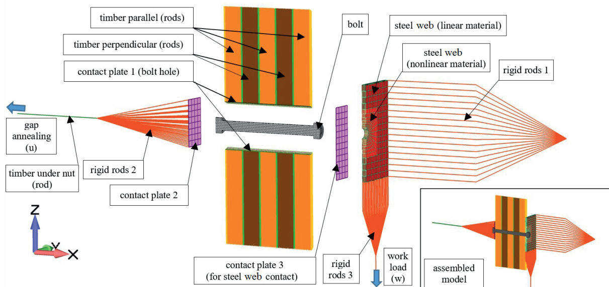
Fig. 7 An exploded view of the connection model, and the assembled connection model (bottom right)
