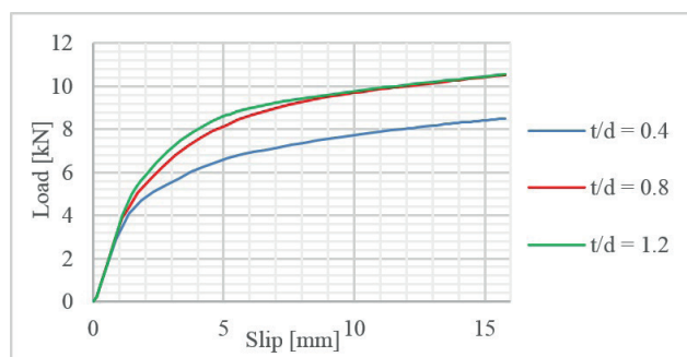
Fig. 25 Load-slip diagram without rope effect
