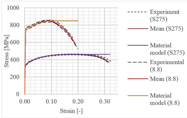
Fig. 8 Experimental stress-strain diagrams for steel material of the profile (S275) and the bolt (8.8)
