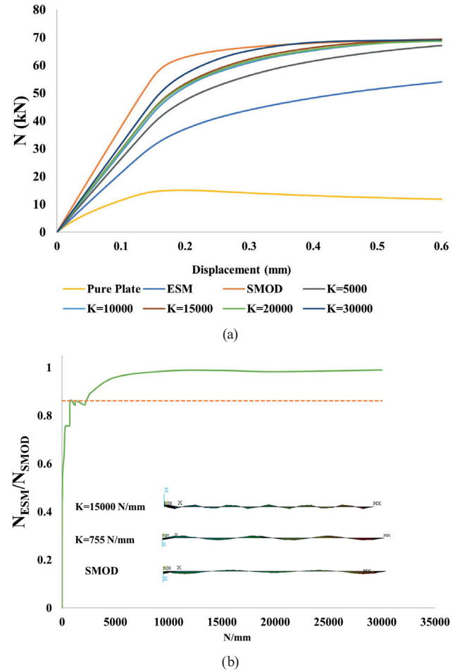
Fig. 12 (a) Load-displacement curve b/t = 250 compression using different K value, (b) spring stiffness sensitivity study
