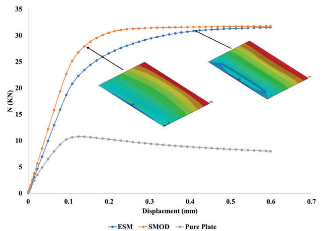
Fig. 10 Load-displacement curves b/t = 175 , E_c = 250 , f_y = 180 MPa ESM spring stiffness calculated based on b/t = 50 constants
