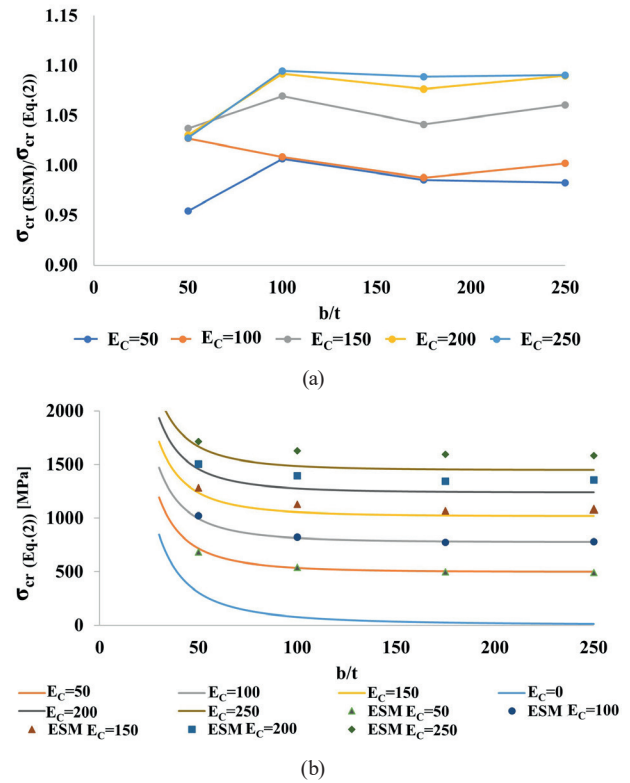
Fig. 5 Verification of ESM, (a) error – b/t relation, (b) Eq. (2) computed stress values as function of b/t considering different elastic moduli versus ESM critical stress results
