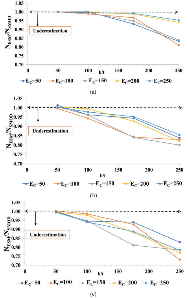
Fig. 9 ESM error using constants corresponding to b/t = 50 in Eq. (1) as function of b/t (a) f_y = 180 MPa, (b) f_y = 280 MPa, (c) f_y = 380 MPa
