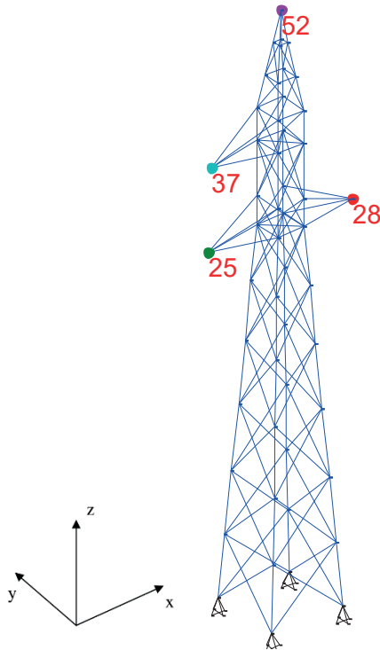
Fig. 5 The layout of 3D truss structure
