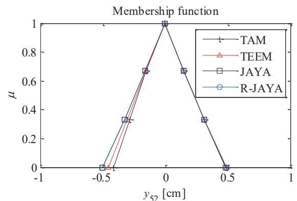
Fig. 7 Membership functions of y_{52} by different methods
