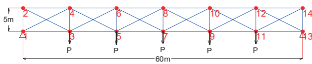
Fig. 1 The layout of 31-bar planar truss
