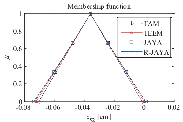
Fig. 8 Membership functions of z_{52} by different methods
