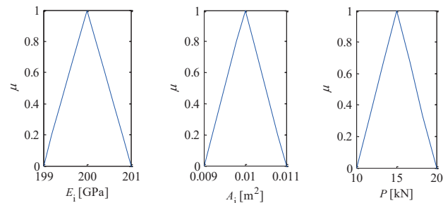
Fig. 2 Membership functions of modulus of elasticity, cross-section area, and load
