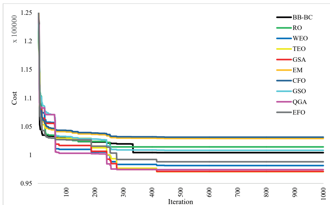
Fig. 2 The mean convergence curves for the CSLP problem obtained by proposed physics-inspired metaheuristic algorithms
