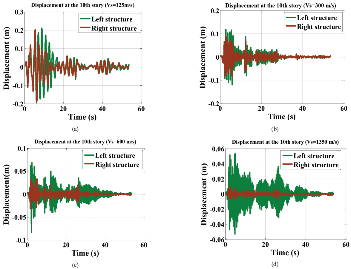
Fig. 7 Displacement time histories for the left and right buildings under different soil types; (a) V_s = 125 m/s, (b) V_s = 300 m/s, (c) V_s = 600 m/s, (d) V_s = 1350 m/s
