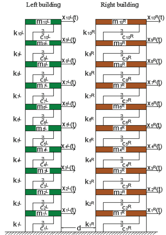
Fig. 2 Model of the two colliding buildings
