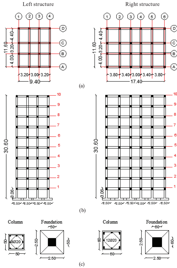
Fig. 5 Description of the selected structure; (a) Plan view, (b) Elevation view, (c) Geometric characteristics for column and foundation
