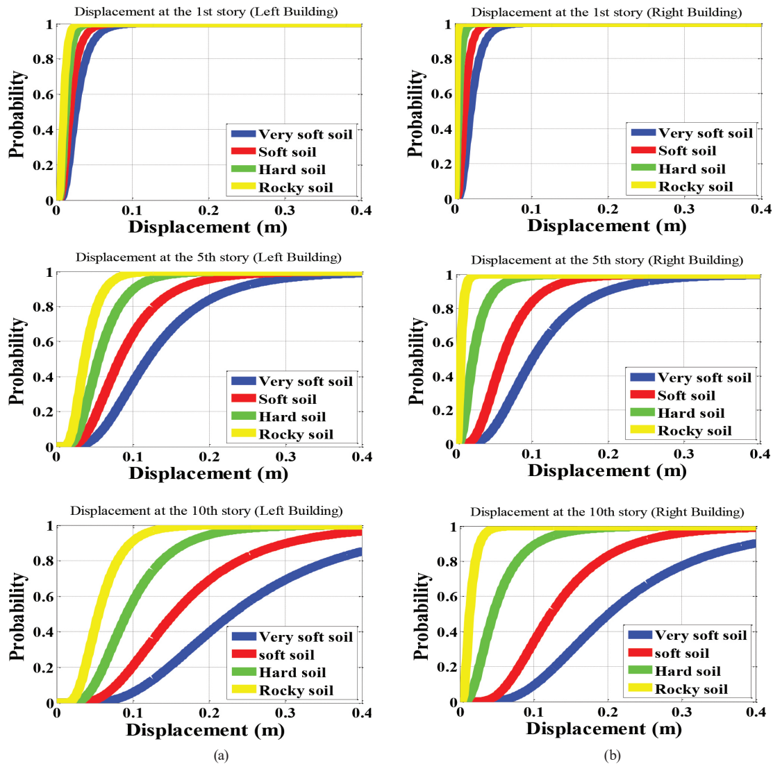
Fig. 9 The displacement probability of the two colliding buildings under different types of soil at the 1 st story, the 5 th story, and the 10 th story; (a) Left building, (b) Right building
