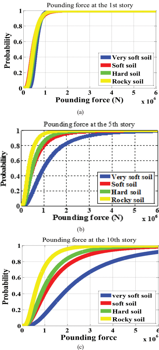
Fig. 10 Probability of the pounding force between colliding buildings under different soil types; (a) at the 1 st story, (b) at the 5 th story, (c) at the 10 th story
