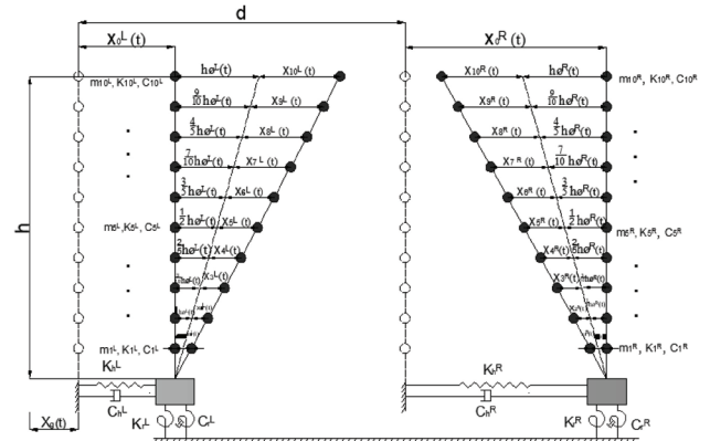
Fig. 3 Model of the two colliding buildings considering SSI
