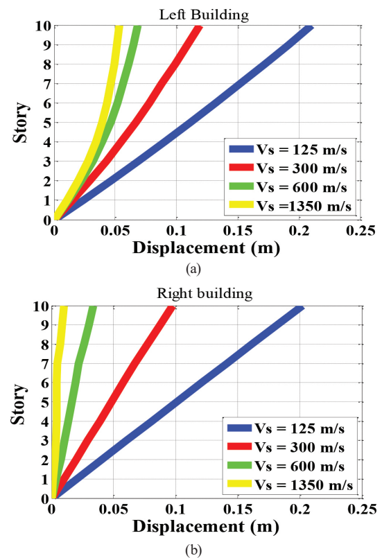
Fig. 6 Peak story displacement at different floor levels of the left and right buildings under different soil types; (a) left structure, (b) right structure
