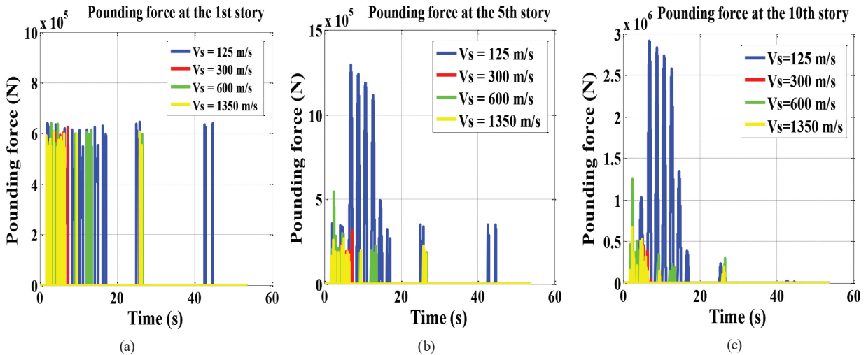
Fig. 8 Pounding time histories for the colliding buildings under different soil types; (a) at the 1st story, (b) at the 5th story, (c) at the 10th story
