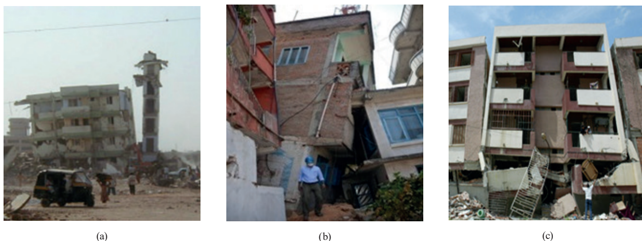
Fig. 1 Examples of buildings that were impacted by pounding in three different earthquakes: (a) Bhuj (2001), (b) Nepal (2015), and (c) Boumerdes (Algeria, 2003)
