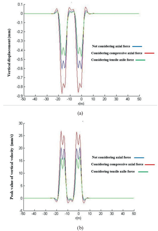
Fig. 5 Output results for rail displacement, sleeper velocity with and without applying compressive and tensile longitudinal force with the value of 1500 [kN] at T = 2.5 [s]
