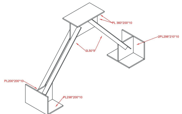
Fig. 2 Detail of eccentric braces used in specimens
