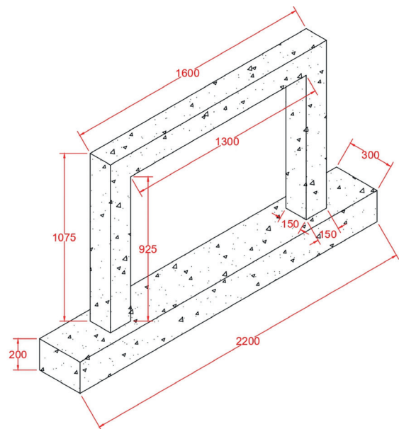
Fig. 1 Details of reinforced concrete frames of experimental samples
