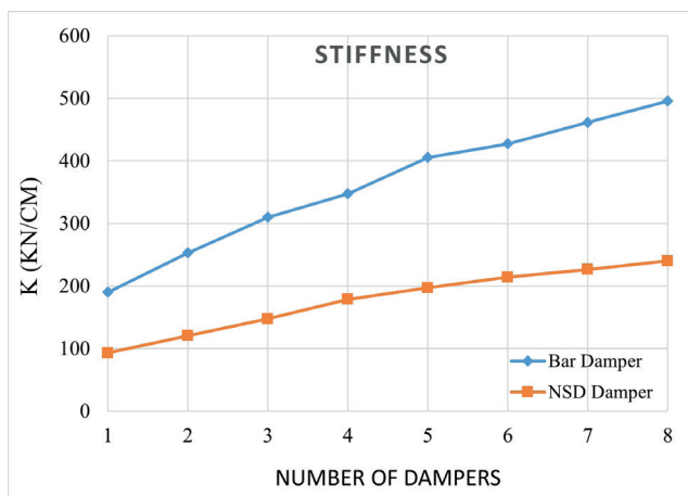
Fig. 11 Diagram of results of numerical models for stiffness parameter
