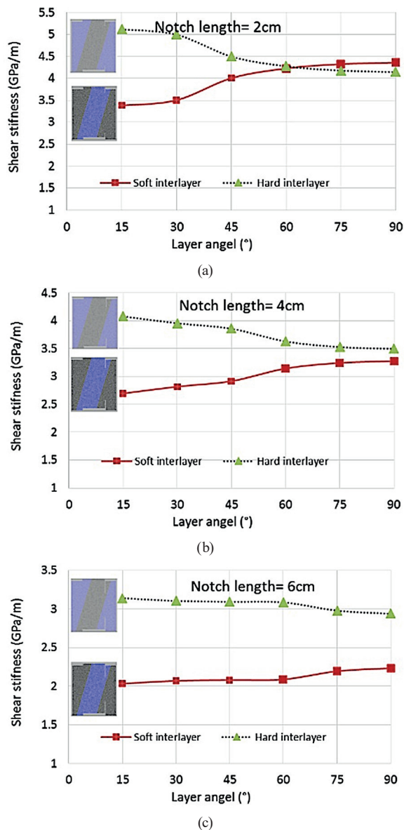
Fig. 6 Effect of layer angle on shear stiffness for notch length of, (a) 2 cm, (b) 4 cm and (c) 6 cm
