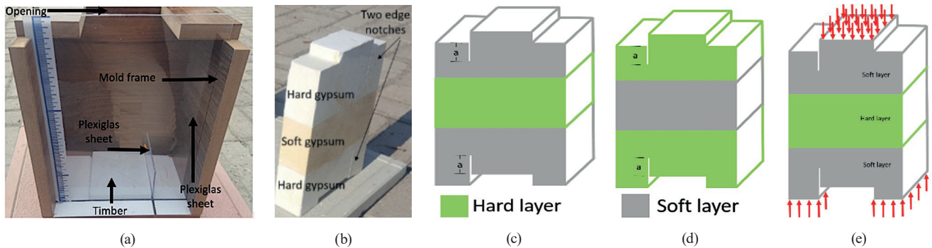
Fig. 3 (a) MDF mold, (b) physical notched layered specimen, (c) three layered model with hard interlayer, (d) three layered model with soft interlayer and (e) notched bedding layer under punch shear test
