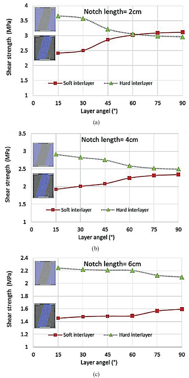
Fig. 8 Effect of layer angle on shear strength for notch length of, (a) 2 cm, (b) 4 cm and (c) 6 cm
