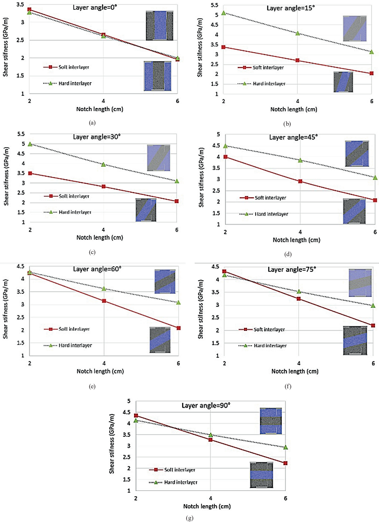
Fig. 7 Effect of notch length on shear stiffness of models with layer angle of, (a) 0°, (b) 15°, (c) 30°, (d) 45°, (e) 60°, (f) 75 and (g) 90°
