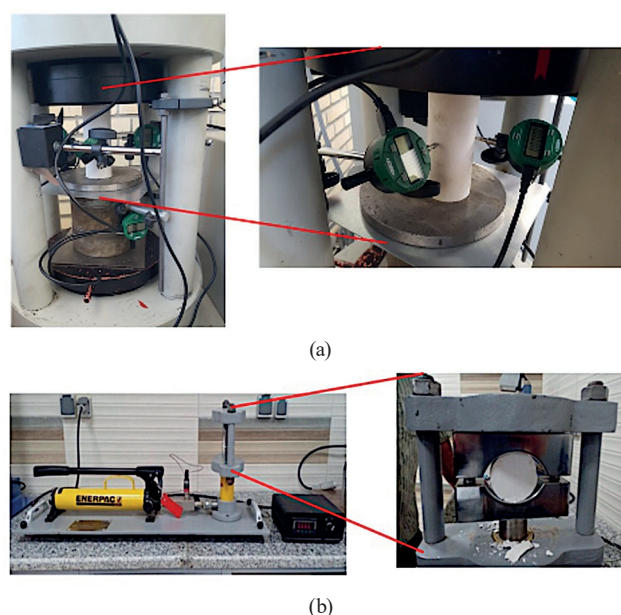
Fig. 2 (a) UCS test and (b) Brazilian test
