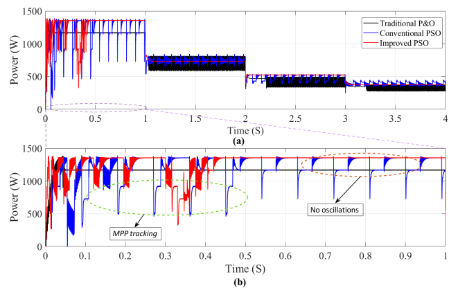
Fig. 9 Output curves of PV string for P&O, PSO and IPSO; (a) Power; (b) Zoom of power
