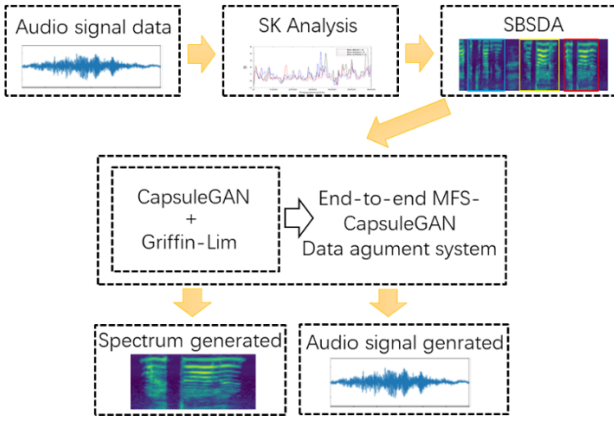
Fig. 5 End-to-end log Mel spectrum data capsule generation countermeasure augmentation system
