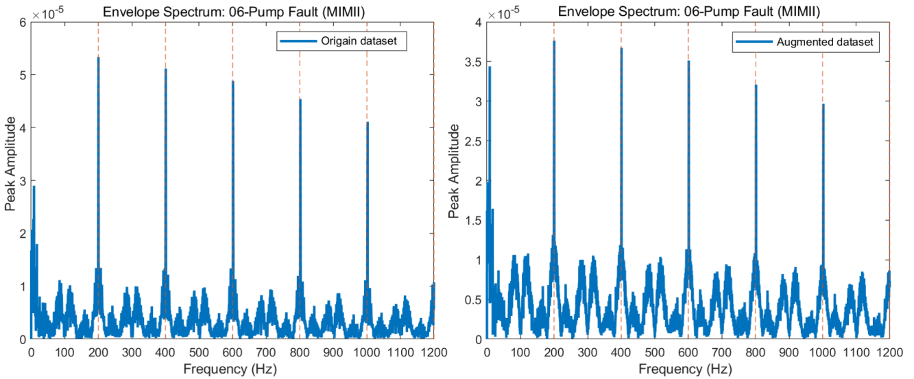
Fig. 18 Comparative analysis of envelope spectrum between the original data and the generated data
