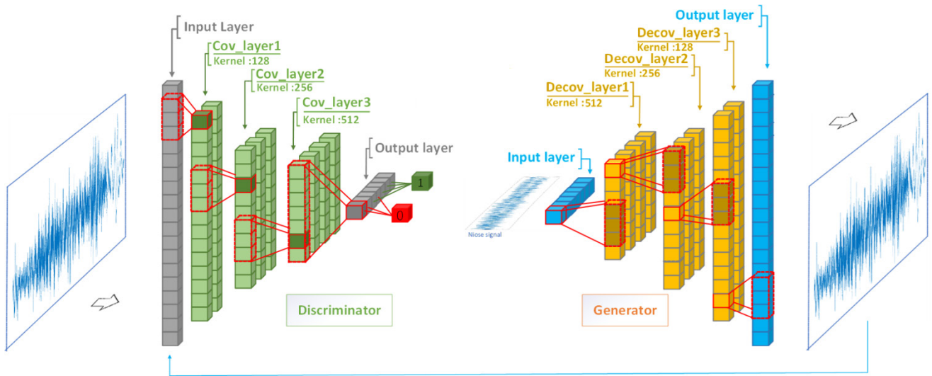
Fig. 4 MFS-DCGAN network diagram: 1 and 0 are tags of normal and abnormal sound, respectively, indicating that the discriminator can distinguish the input sound samples from real data or fake data generated by MFS-DCGAN
