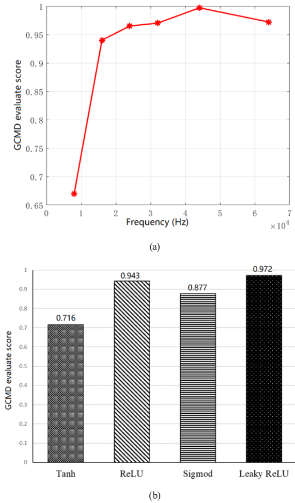
Fig. 15 (a) Accuracy of GCMD model after training with datasets of different sampling frequencies, (b) Influence of different activation functions on GCMD network
