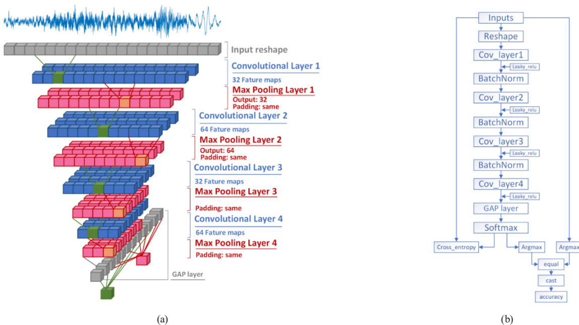
Fig. 7 CNN model architecture for Abnormal Sound Detection of Machines. (a) The detailed composition of each CNN layer structure, (b) CNN's tensor flow diagram and the modes of activation added to each layer
