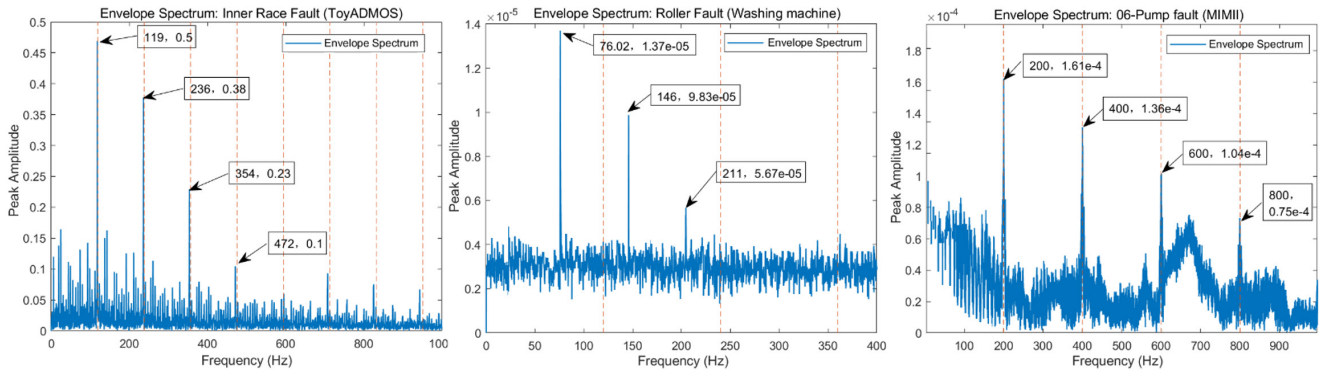
Fig. 10 Spectrum envelope analysis diagram of fault signal
