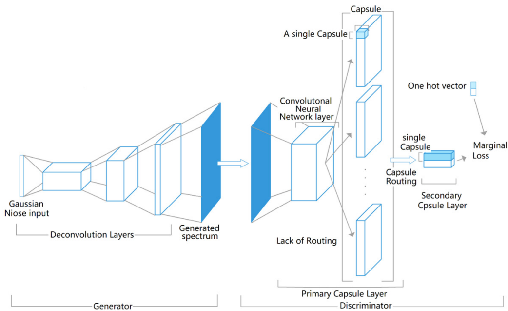
Fig. 6 MFS-CapsuleGAN model
