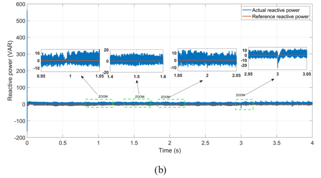
Fig. 11 Active and reactive power behavior using Backstepping-LQR controller with M variation
