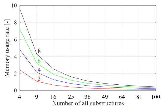
Fig. 9 The rate of convergence decreases for an increasing number of predefined substructures
