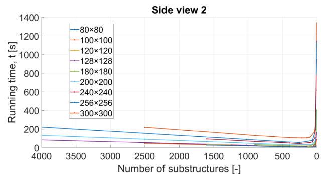
Fig. 11 Variation of running time of constant degree of freedom curves as a function of reduction ratio and the number of substructures
