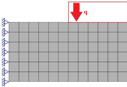
Fig. 1 Boundary conditions of the meshed plate
