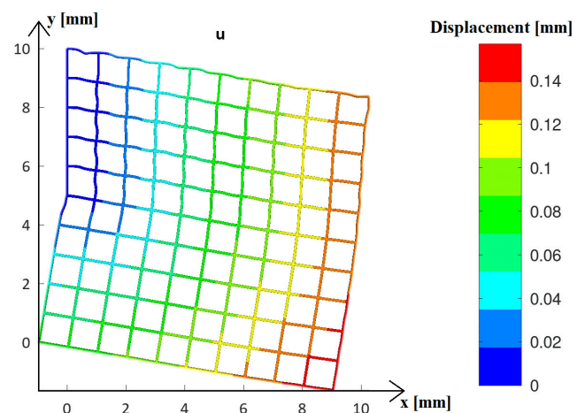
Fig. 6 Model displacement field built from substructures
