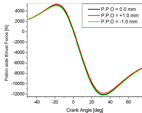
Fig. 7 Effect of the piston pin offset on the piston side thrust force
